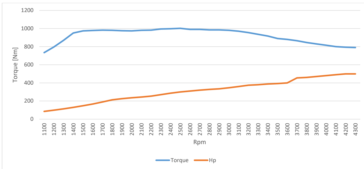
Diemmax V12-520 engine Power curve
